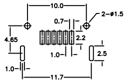
P.C. Board Layout (Top View)
